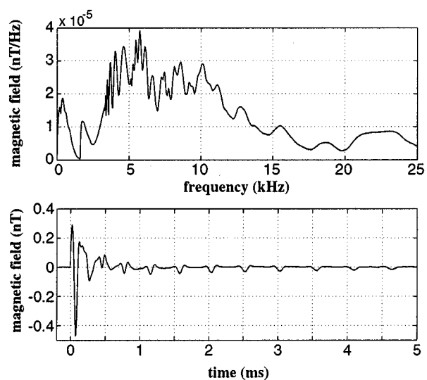
Fig. 3. Sample mode theory calculation for a transient source 1000 km from the receiver. (a) Magnetic field amplitude as a function of frequency. (b) Magnetic field waveform as a function of time, calculated with a numerical inverse Fourier transform.
