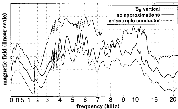
Fig. 5. Nighttime ELF-VLF spectra computed with mode theory for different ionospheric approximations. Note the nonlinearity of the horizontal scale. The curves are offset by one grid unit each.
